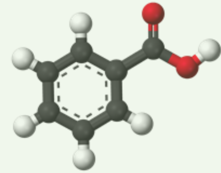
Benzoic Acid
