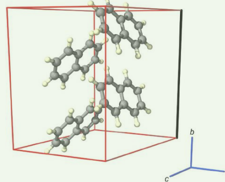
Naphthalene
